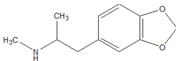
N-Methyl-3,4-methylenedioxyamphetamine (MDMA)
