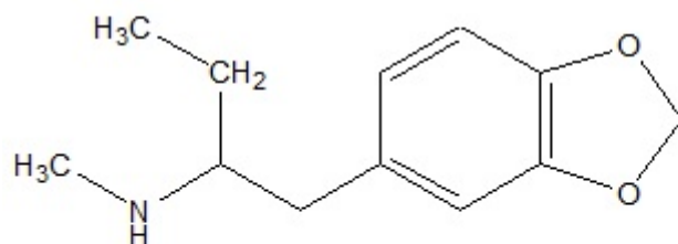
N-Methyl-1-(3,4-methylenedioxyphenyl)-2-butanamine (MBDB)
